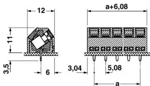
Dimensioned drawing
